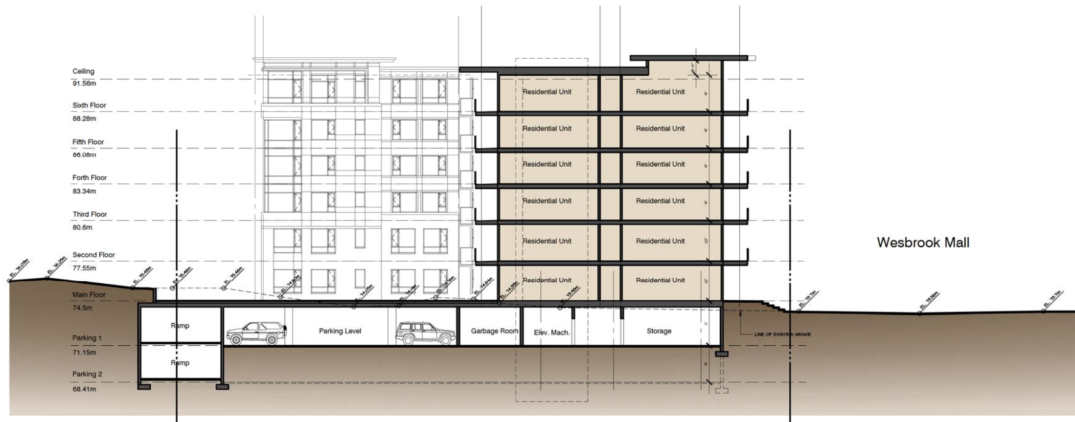
Section BB ~ East-West through Lobby
