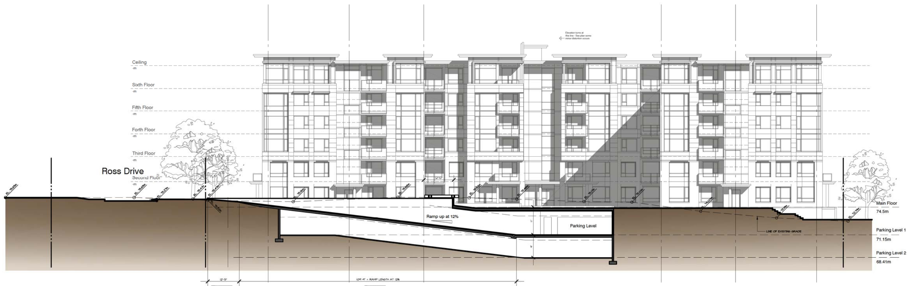
Section AA ~ North South through Parking Ramp
