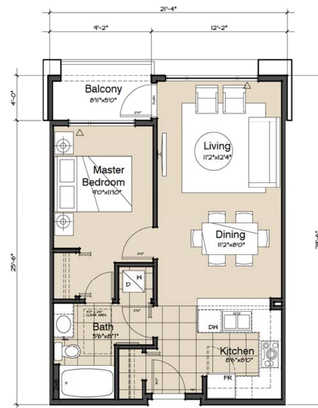
Unit E One Bedroom Area: 580 sf 6 of 94 units
