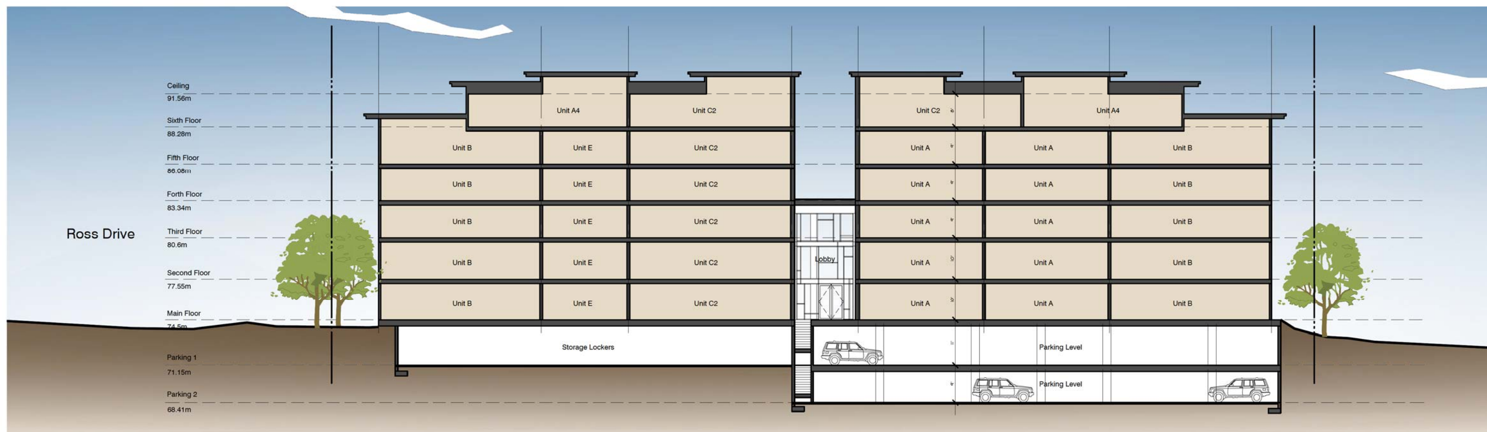
Section CC ~ North - South through Lobby
