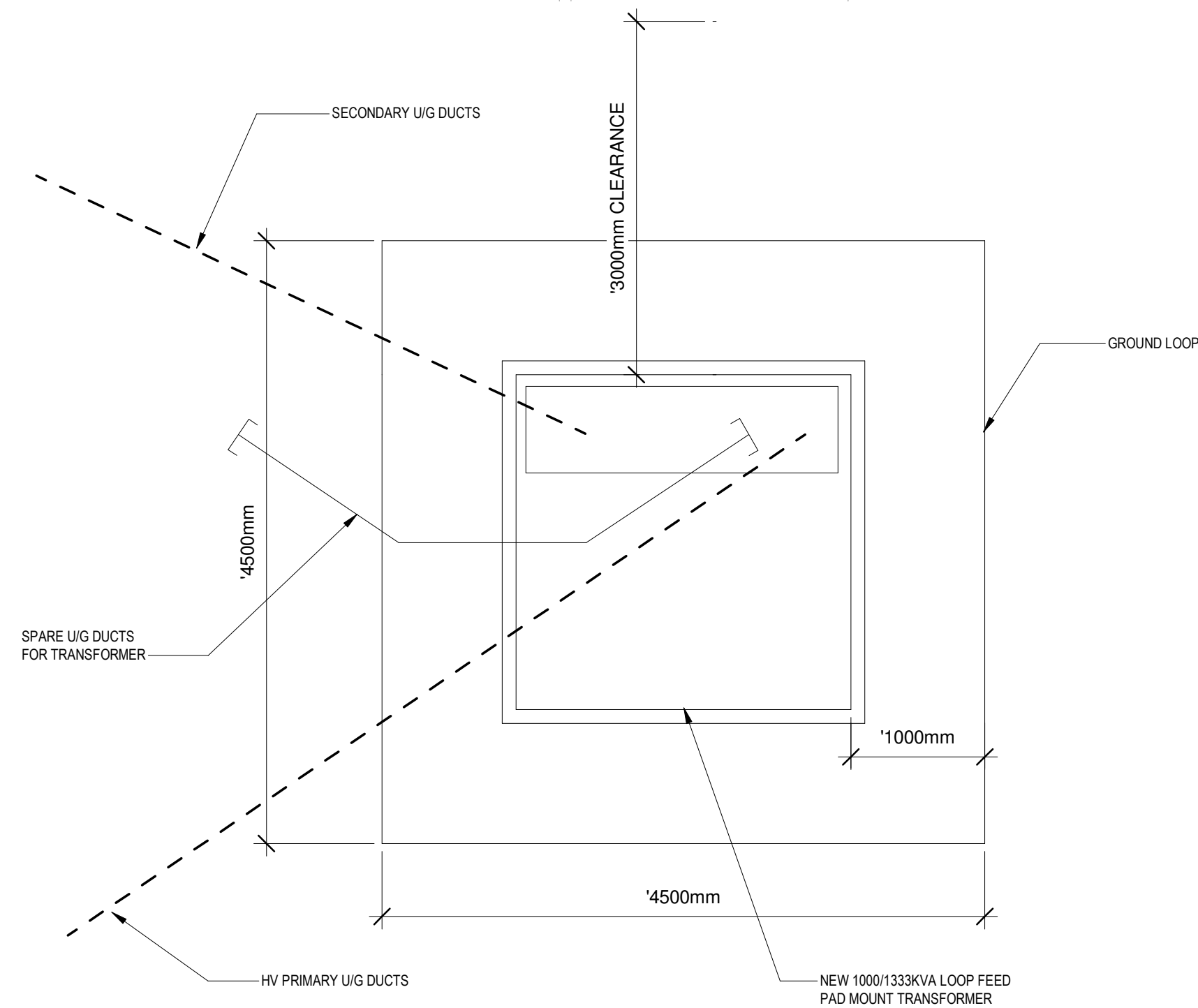
2 LOOP FEED PAD MOUNTED TRANSFORMER DETAIL NTS
